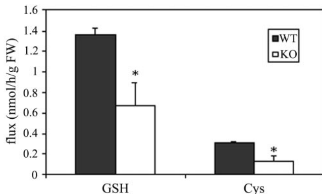
FIG. 6. Incorporation of ^{35}\text{S} from ^{35}\text{S} sulfate into thiols. Wild type moss and the 11-3-12 \Delta apr knockout were incubated in Knop's medium containing 0.06 mM sulfate supplemented with ^{35}\text{SO}_4^{2-} for 2 h. Radioactive sulfur in cysteine and GSH was measured. Mean values \pm S.D. from three measurements are presented. Values indicated by asterisks are different at p \leq 0.005 .
